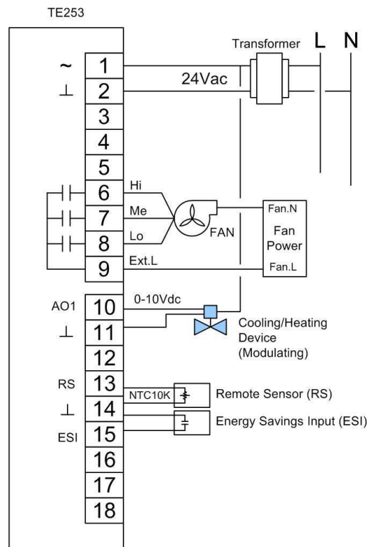
Wiring diagram for TE253 thermostat
